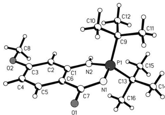
Figure 1. Structure of compound 5e in the crystal.
